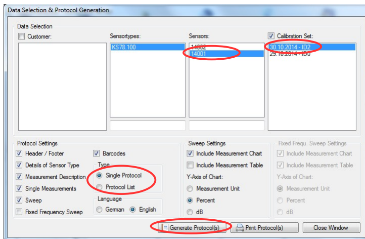
Figure 48: Protocol Generation
