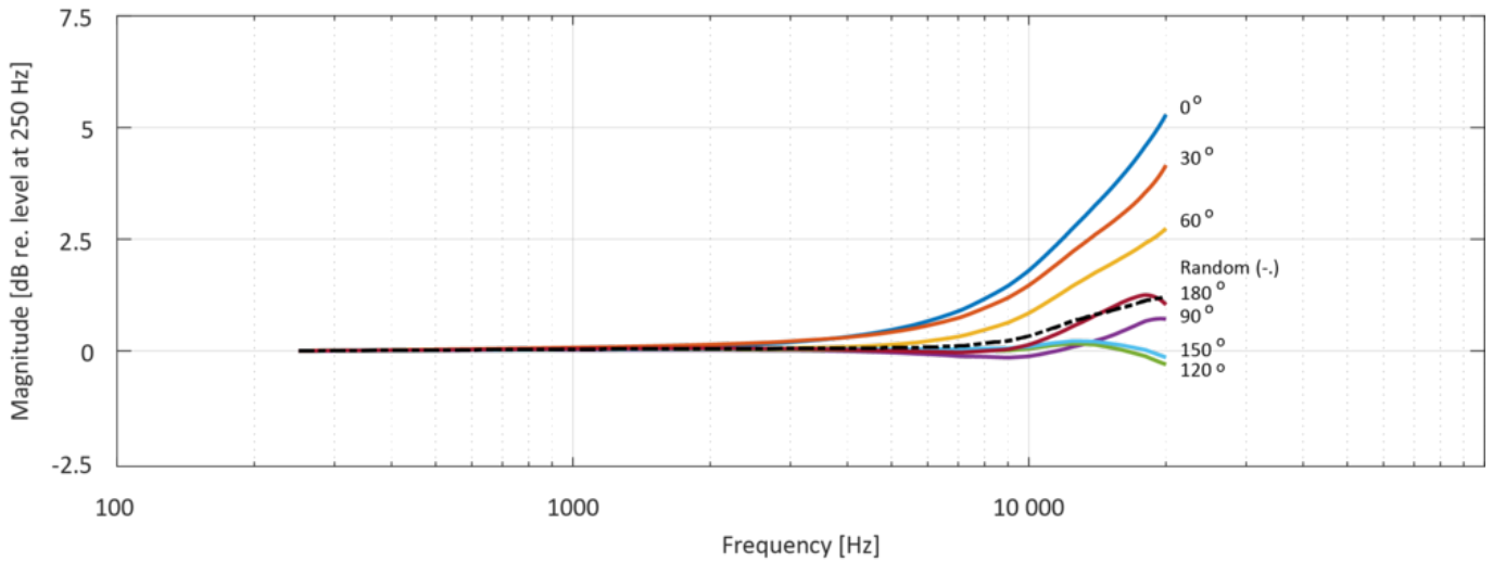
Free-field corrections for different angles of incidence with grid
