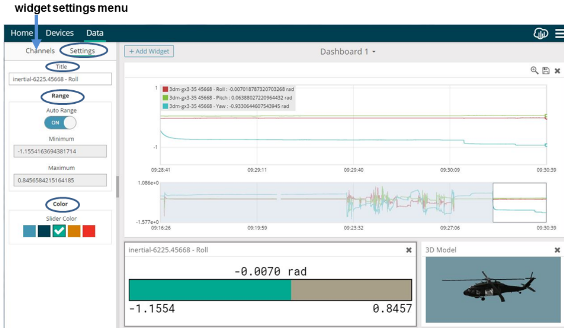
Figure 43 - Widget Settings Menu
