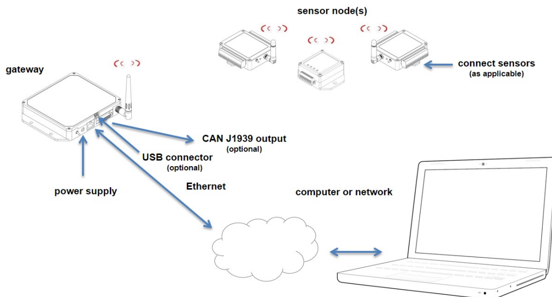
Figure 4 - System Connections
