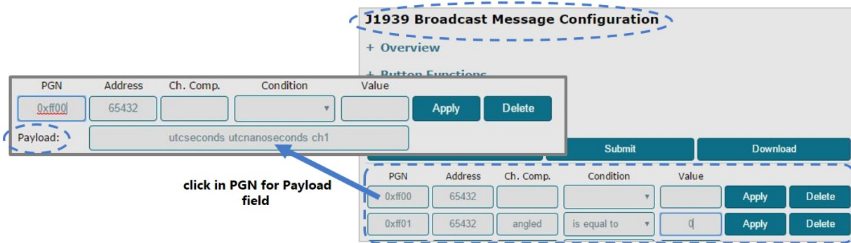
Figure 15 - Broadcast Message Menu Example
