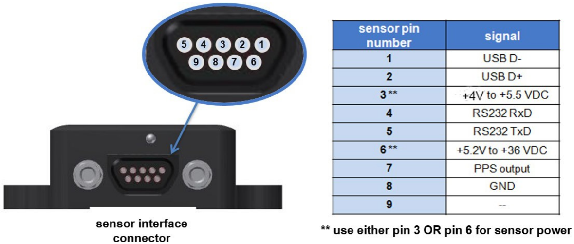
Figure 37 -Connector Wiring
