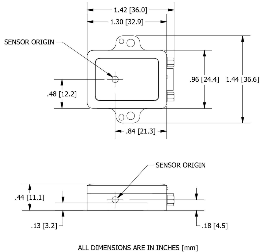
Figure 40 - 3DM-GX5-25 Sensor Origin
