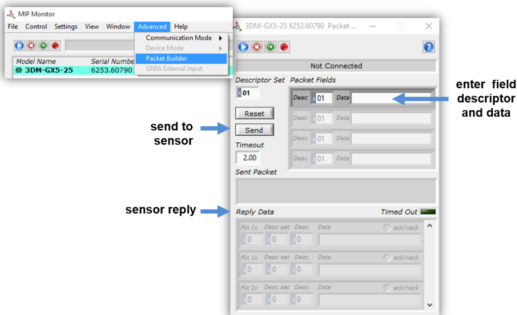
Figure 35 -Packet Builder
