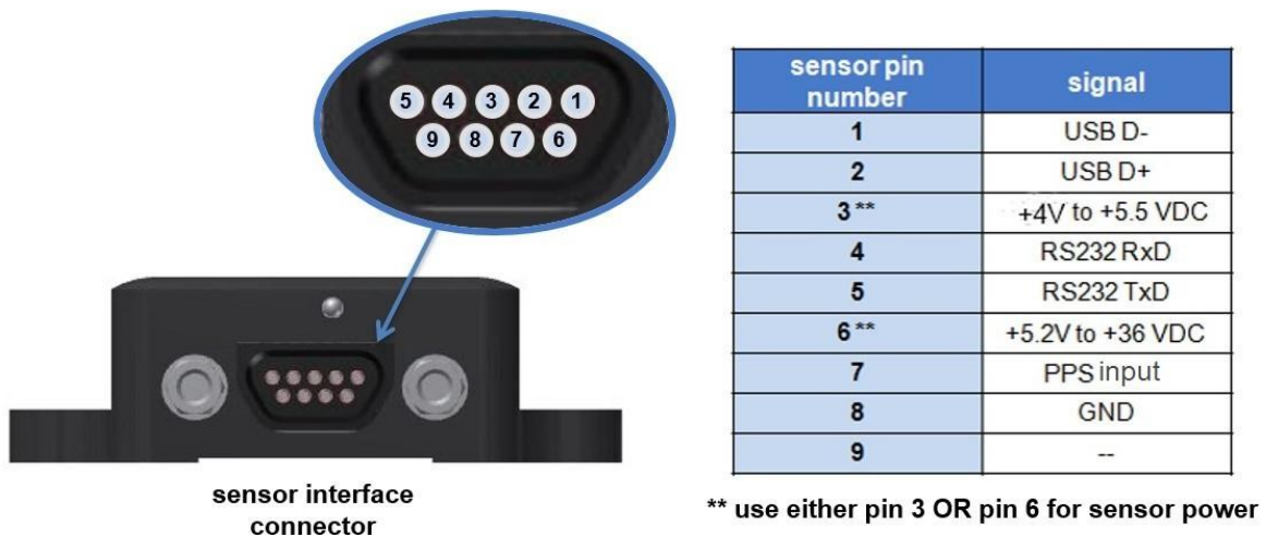
Figure 37 -Connector Wiring
