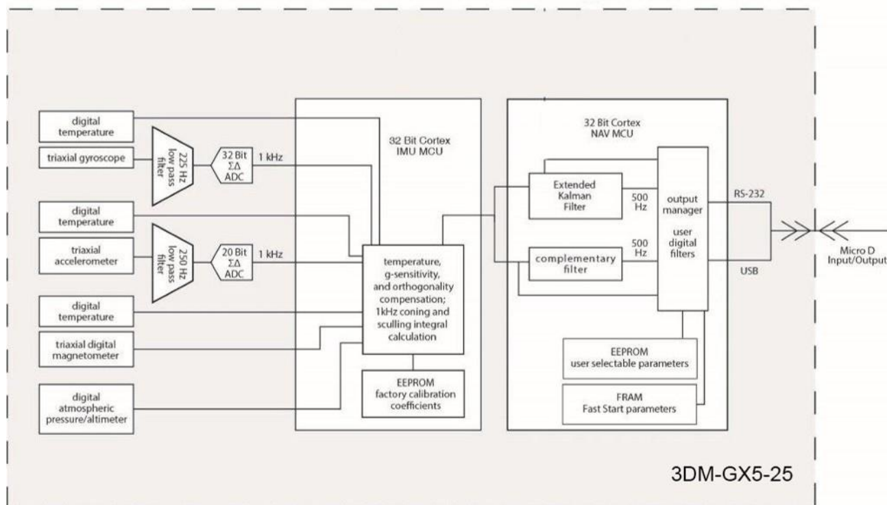
Figure 14 -3DM-GX5-25 Block Diagram
