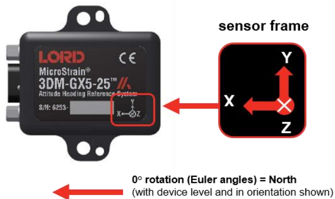
Figure 19 -Sensor Frame
